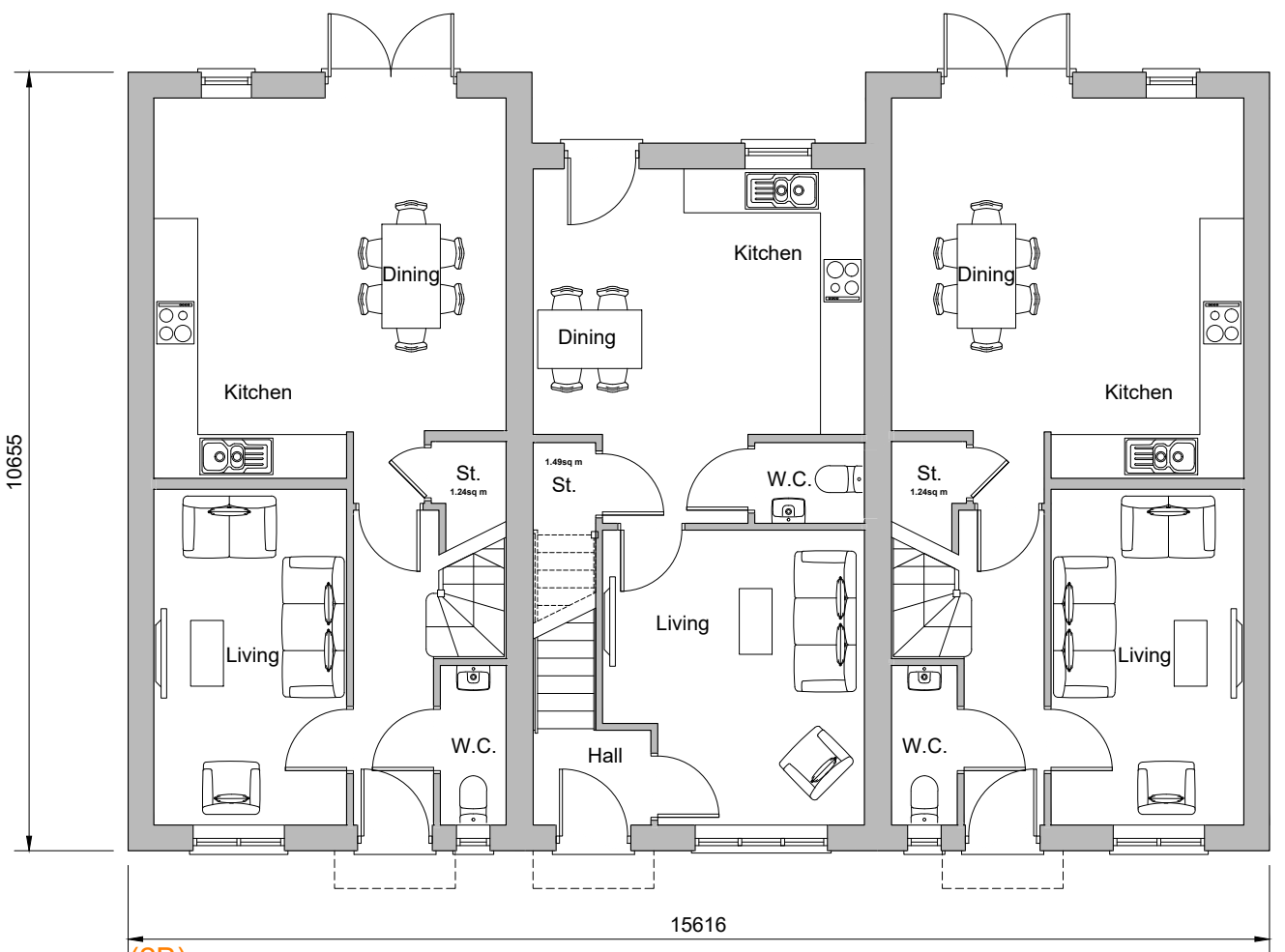
Ground Floor Plan Plots 20-22
