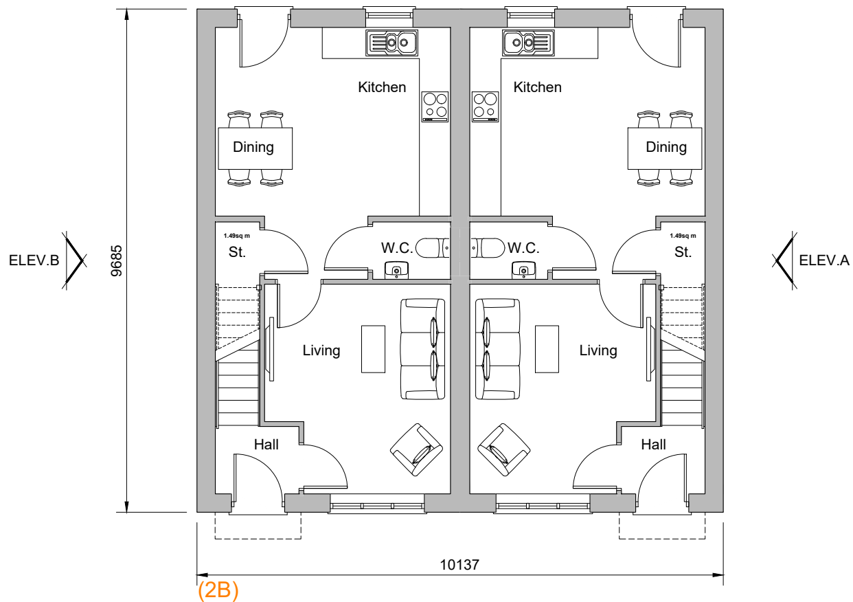
Ground Floor Plan Plots 5-6, 7-8, 11-12, 43-44 & 45-46
