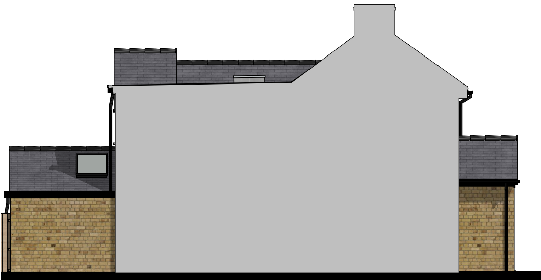
1:100 Proposed North Elevation
