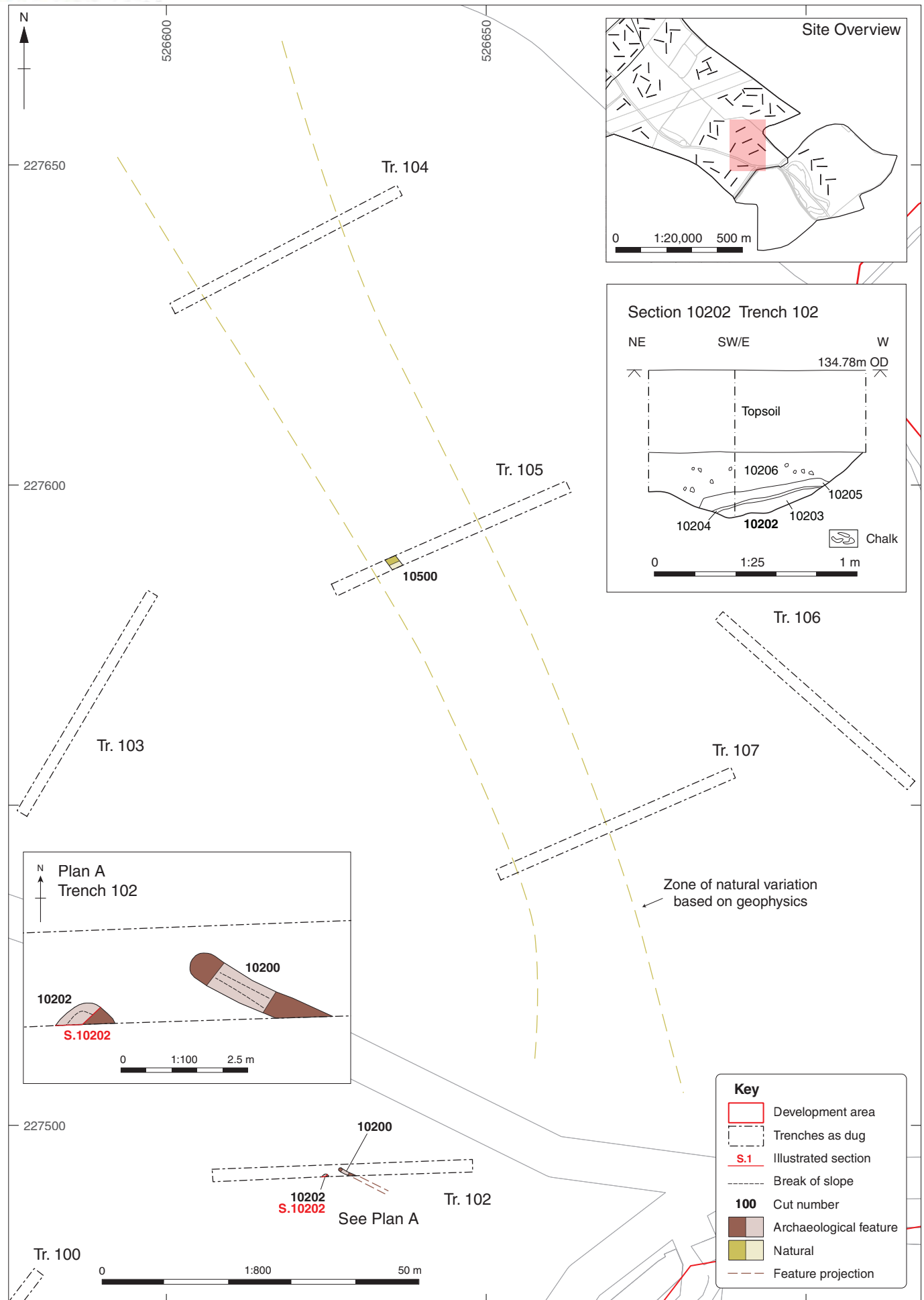
Figure 7: Trenches 102-107
