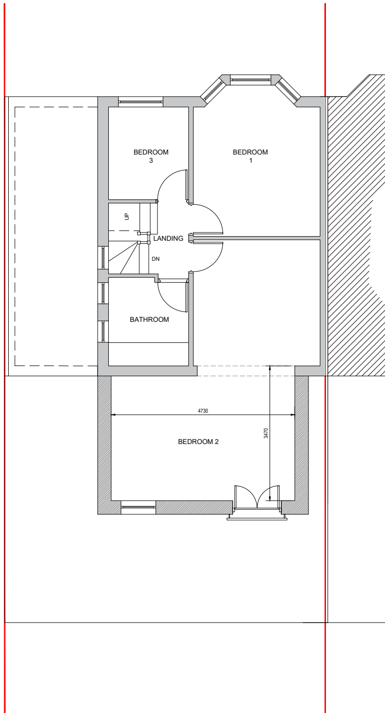
FIRST FLOOR PLAN AS PROPOSED, 1:100 @ A3
