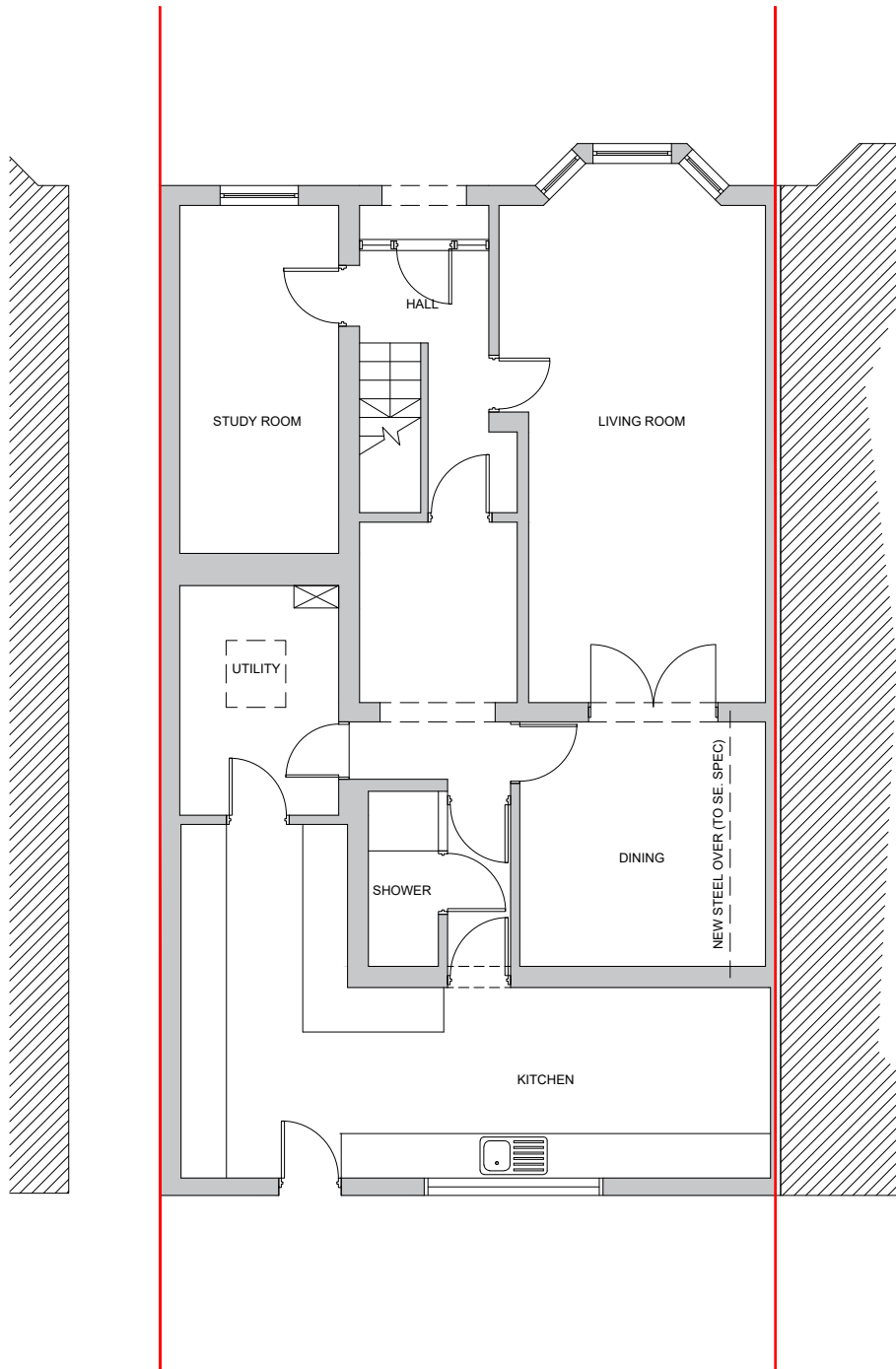
GROUND FLOOR PLAN AS PROPOSED, 1:100 @ A3
