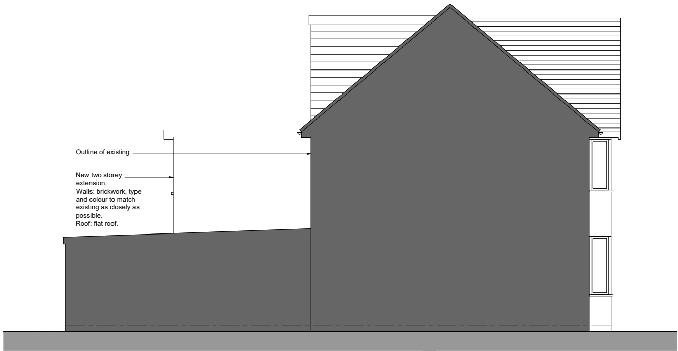
SIDE ELEVATION AS PROPOSED, 1:100 @ A3
