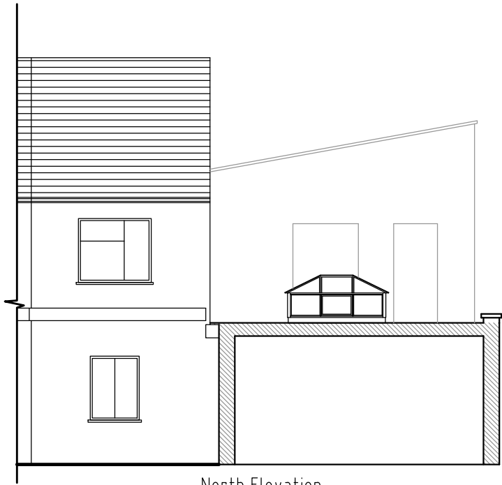
North Elevation
