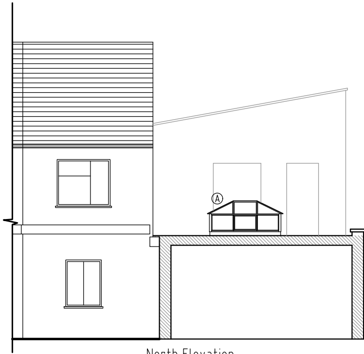
North Elevation
