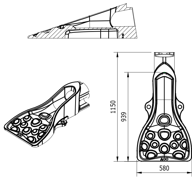
ACO SWALE INLET FOR 1500 PIPES SCALE 1:20
