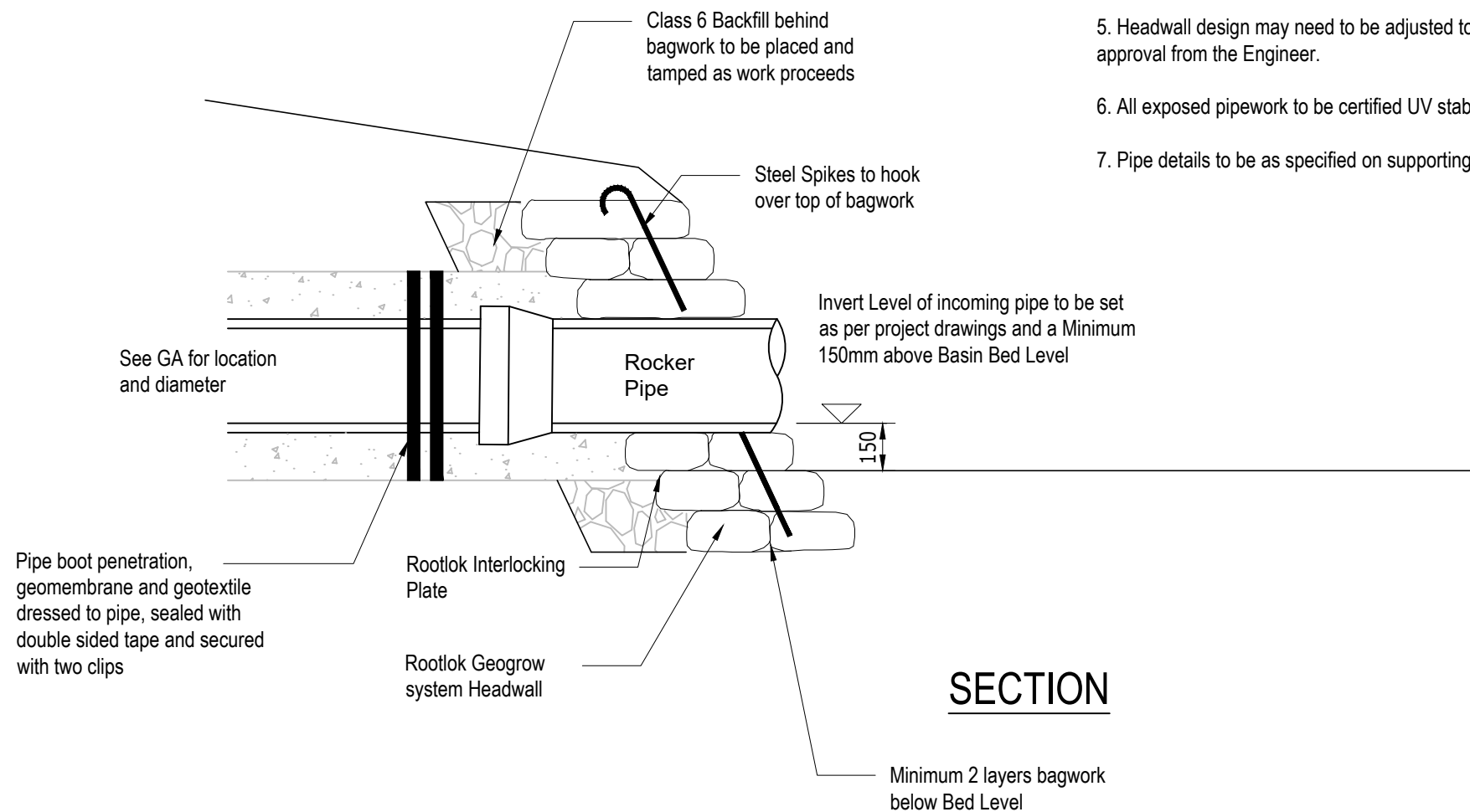
BAGWORK HEADWALL FOR 225mm - 375mm PIPES SCALE 1:20
