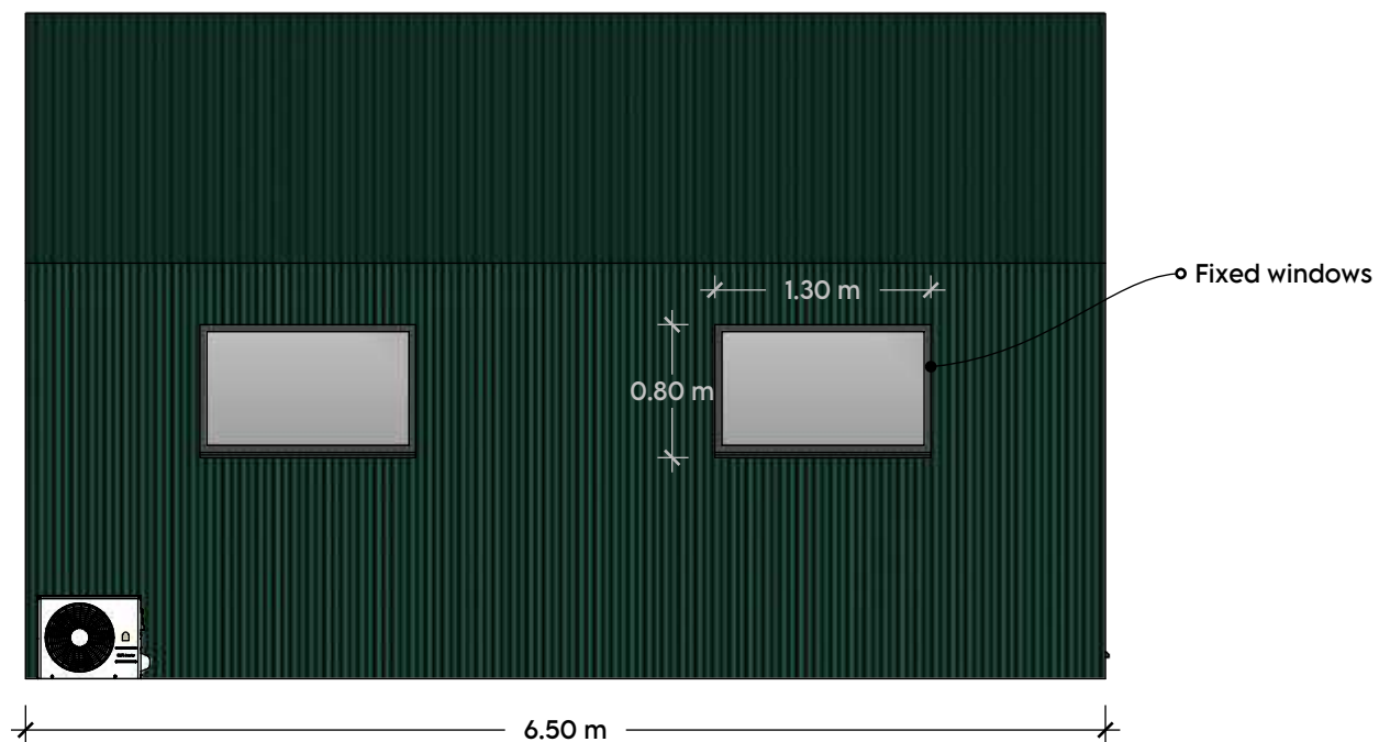
Rear Elevation
