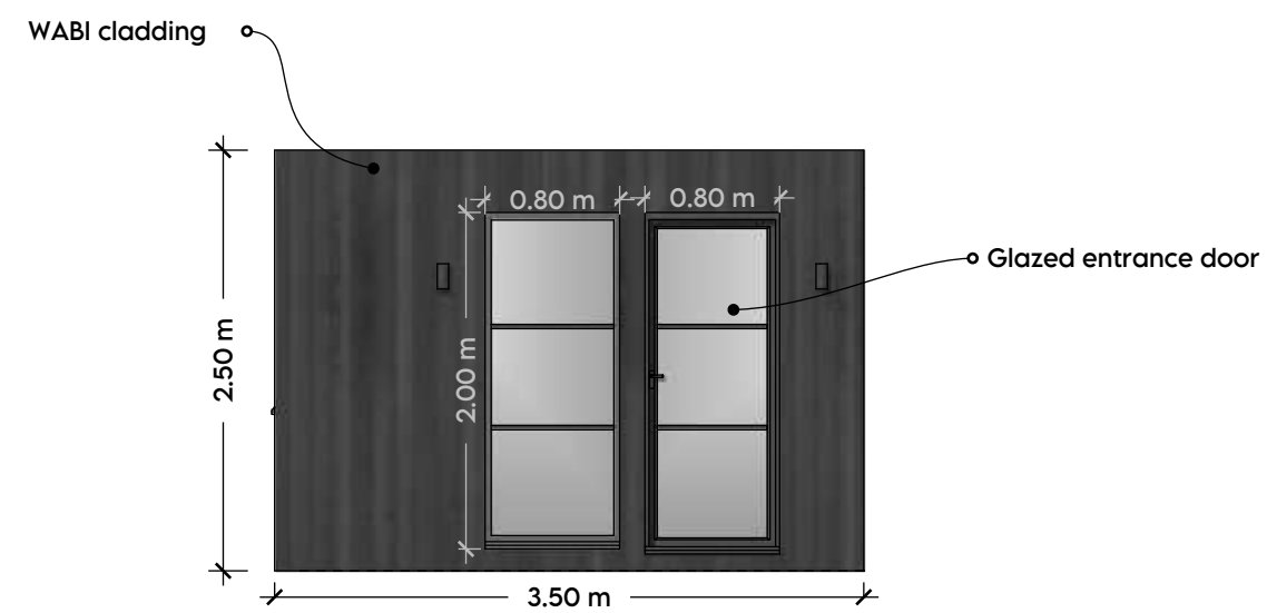
Front Elevation
