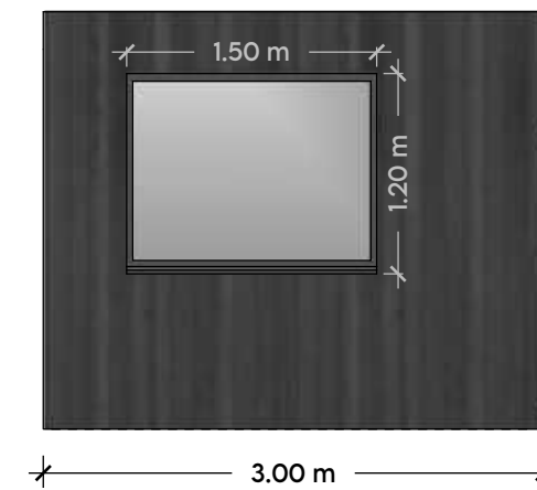
Left Elevation
