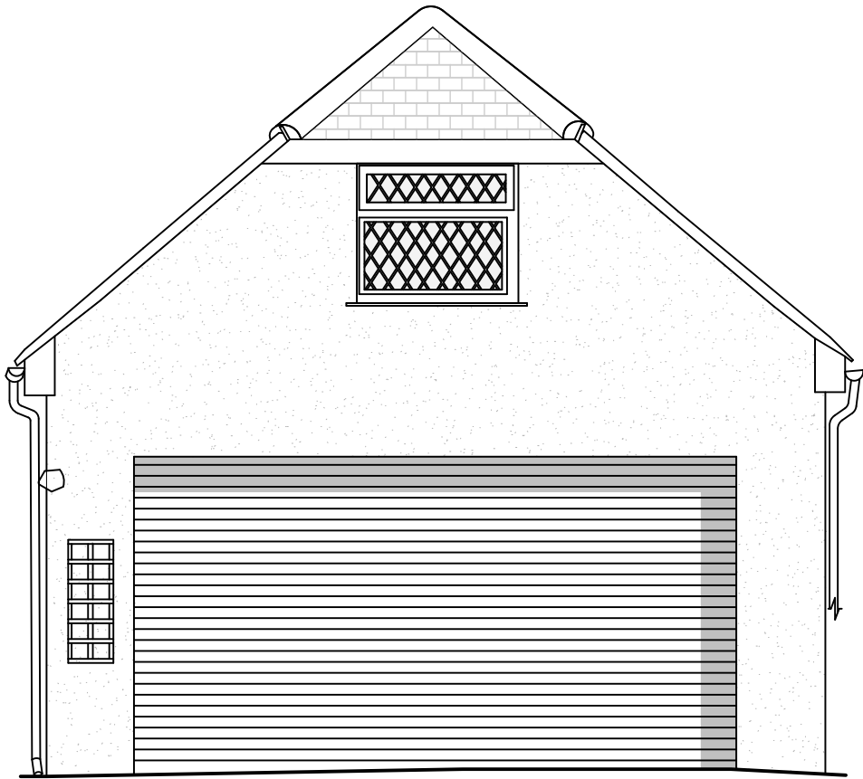
Front Elevation 1:50
