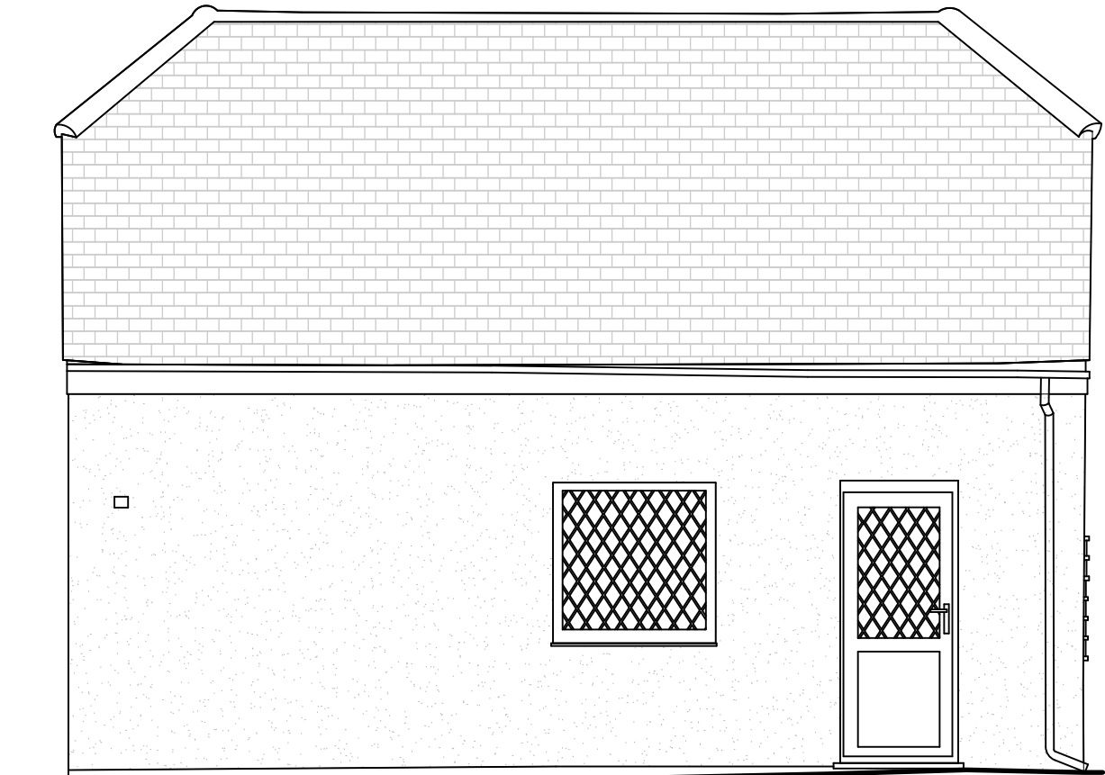
Side Elevation 1:50
