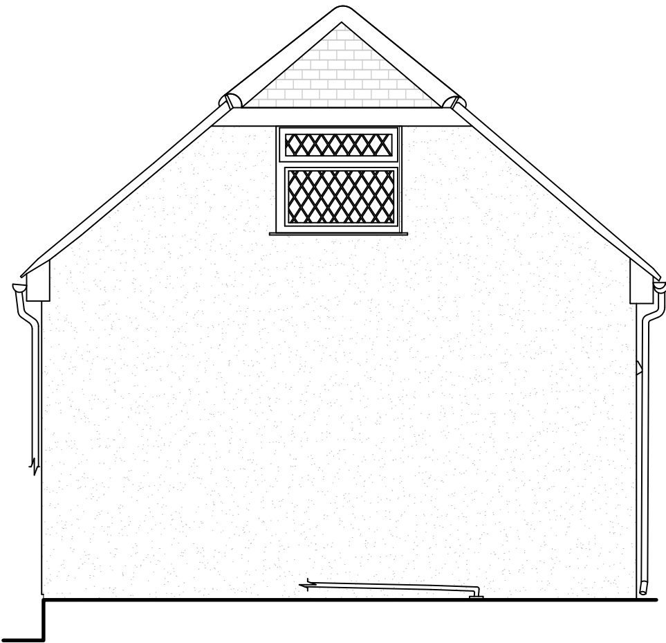
Rear Elevation 1:50
