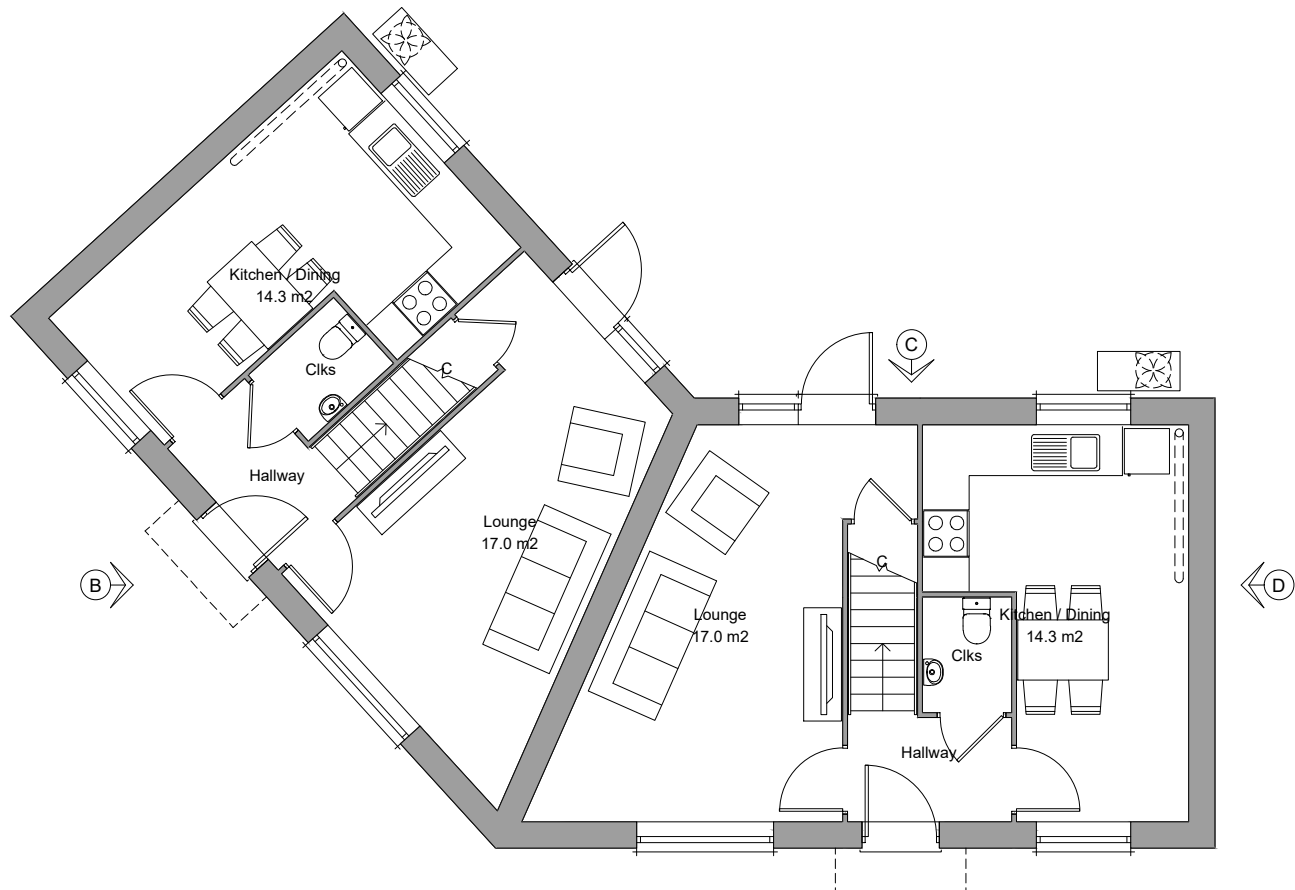
Ground Floor Plan Area 40.2m²
