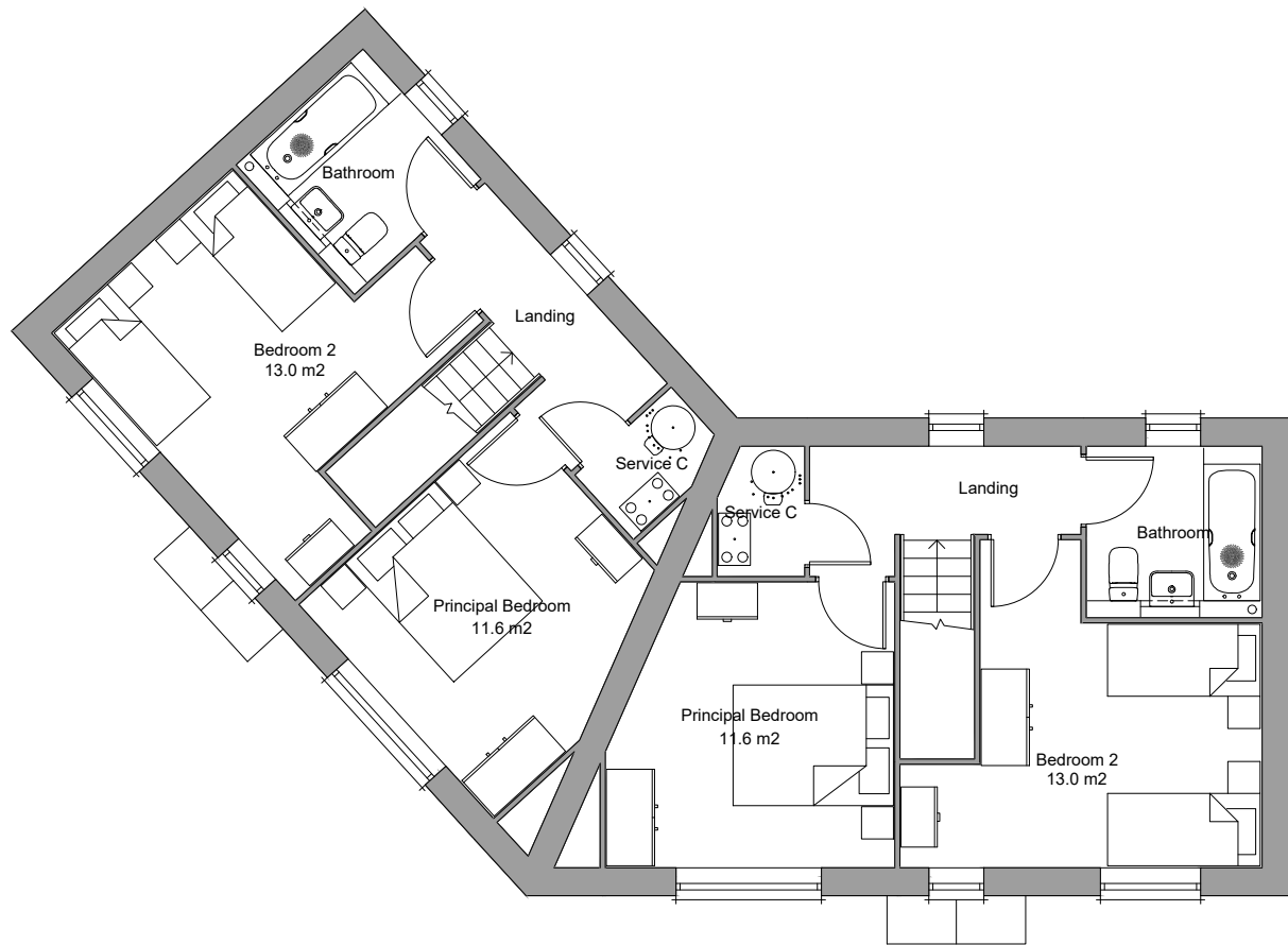
First Floor Plan Area 40.2m²
