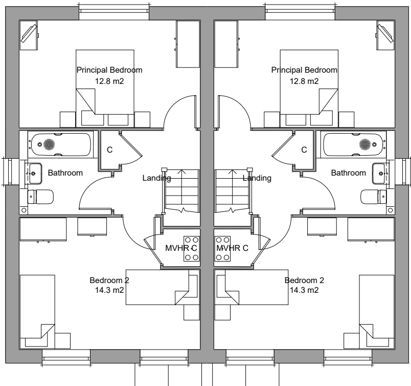
First Floor Plan Area 40.0m²
