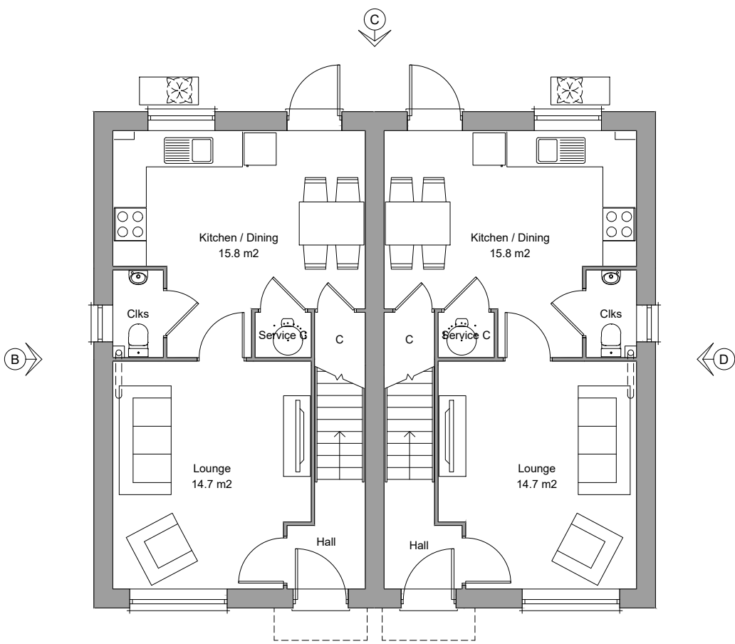
Ground Floor Plan Area 40.0m²
