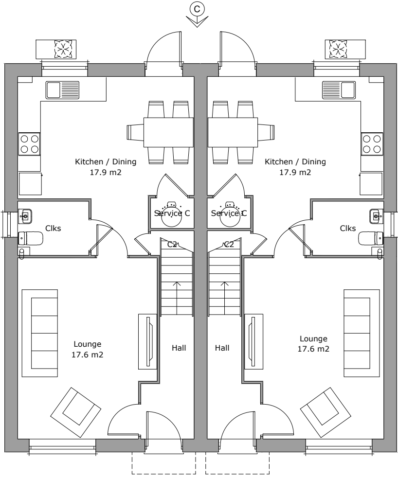
Ground Floor Plan Area 47.4m²
