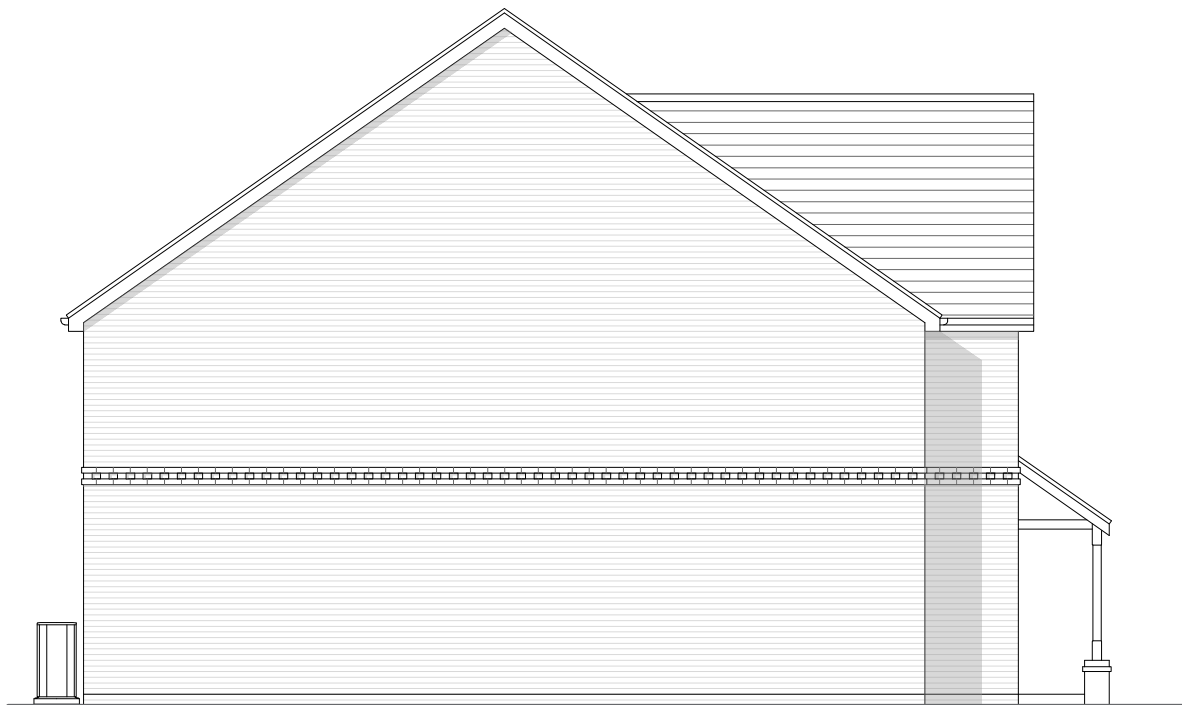
Elevation D
