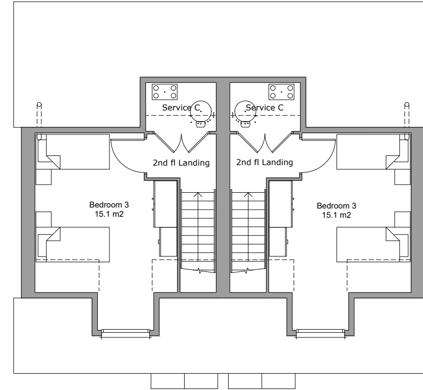
Second Floor Plan Area 23.2m²
