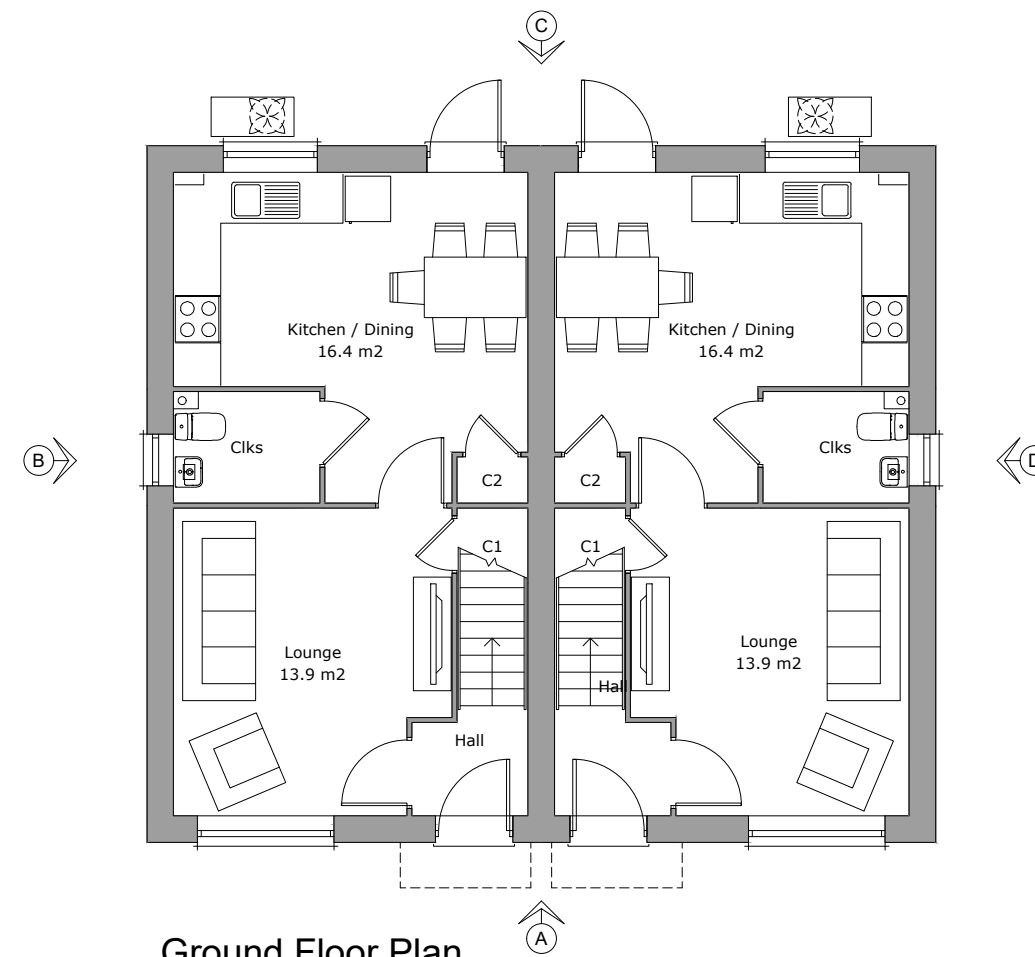
Ground Floor Plan Area 40.0m²
