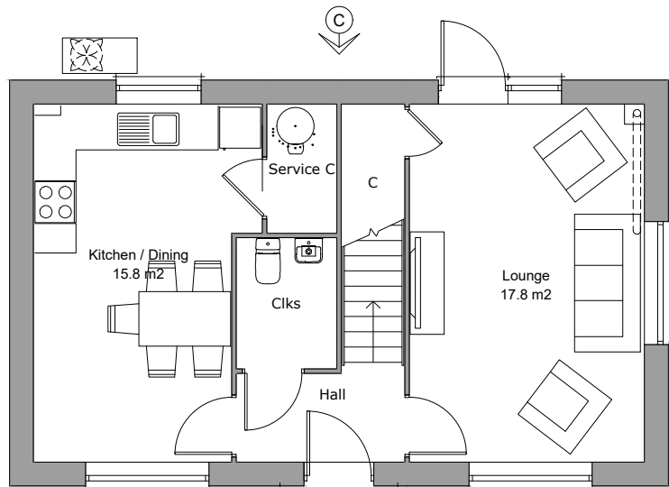
Ground Floor Plan Area 47.1m²
