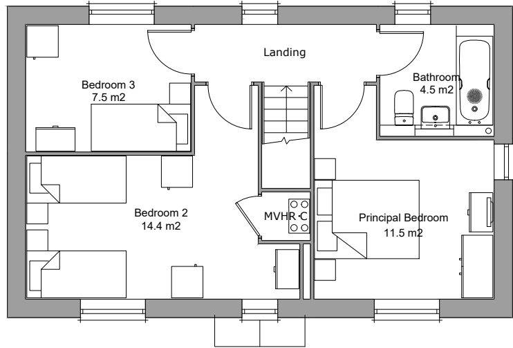
First Floor Plan Area 47.1m²
