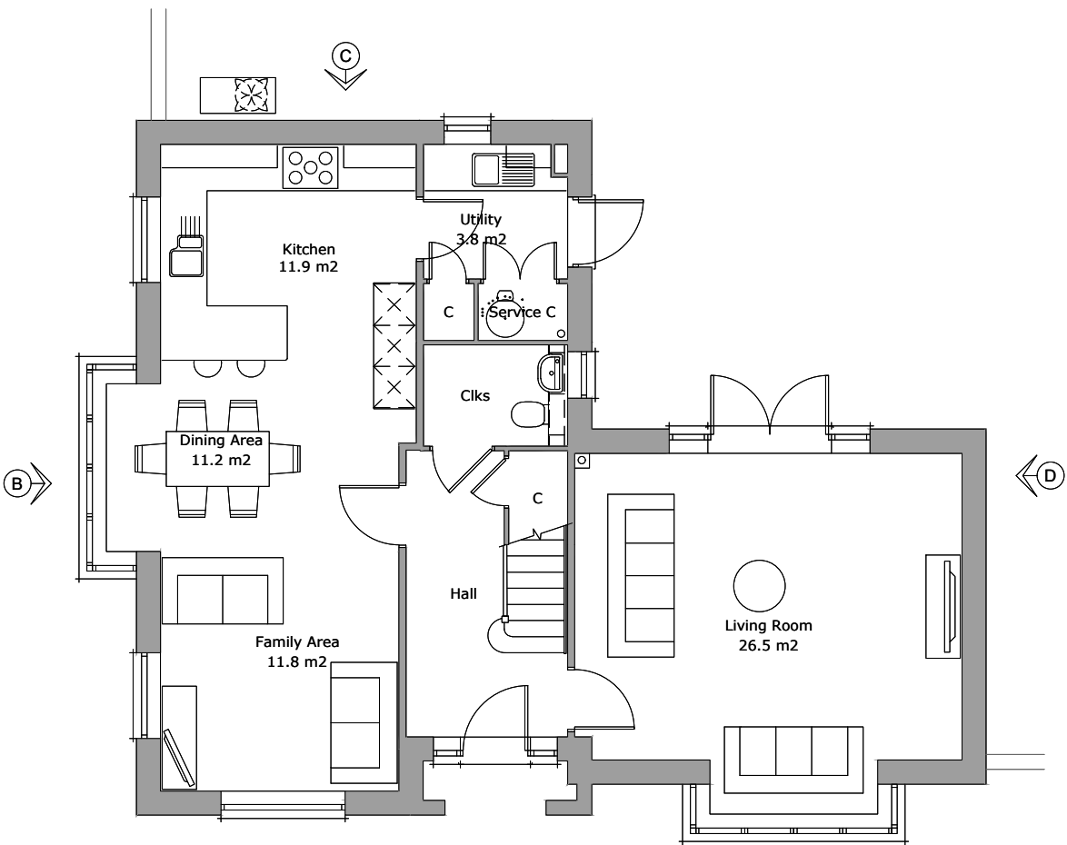
Ground Floor Plan Area 83.5m 2
