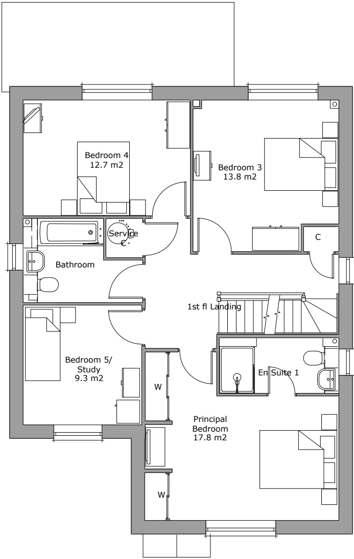
First Floor Plan Area 81.1m 2
