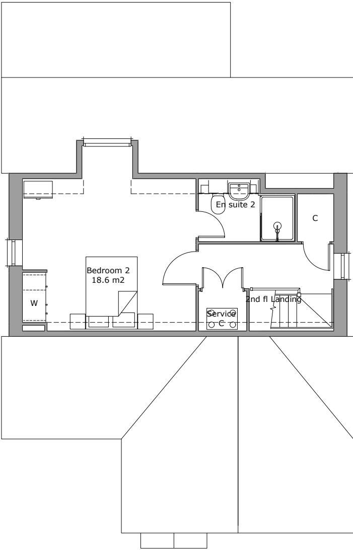
Second Floor Plan Area 33.2m 2
