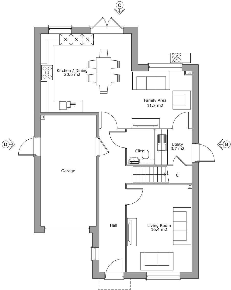
Ground Floor Plan Area 71.7m 2
