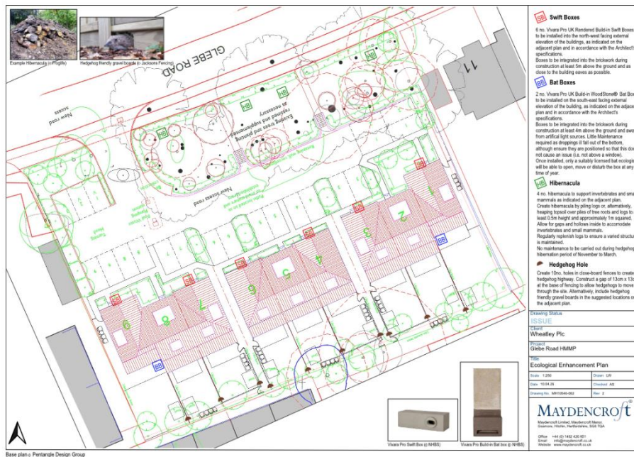
Figure 5: Bat Boxes Details
