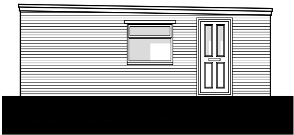
PROPOSED SIDE ELEVATION (D-D)
