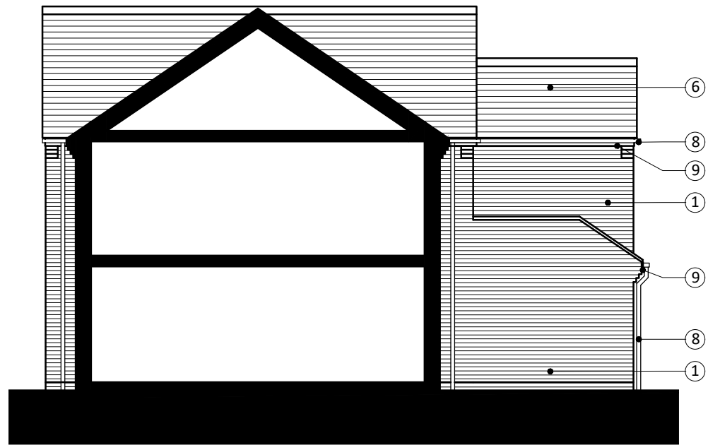
SIDE ELEVATION (C-C)
