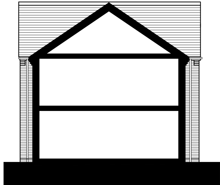
SIDE ELEVATION (C-C)
