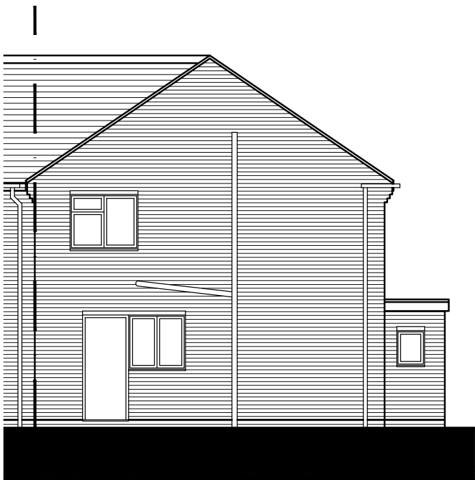
REAR ELEVATION (B-B)
