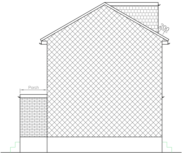
PROPOSED RIGHT SIDE ELEVATION
