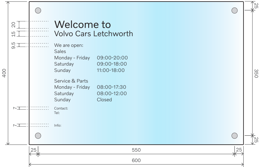
FRONT ELEVATION scale 1:5
