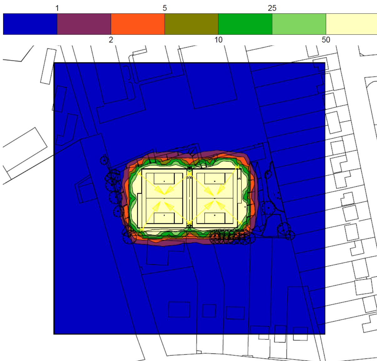
Figure 6 – Floodlighting Illuminance (Lux)
