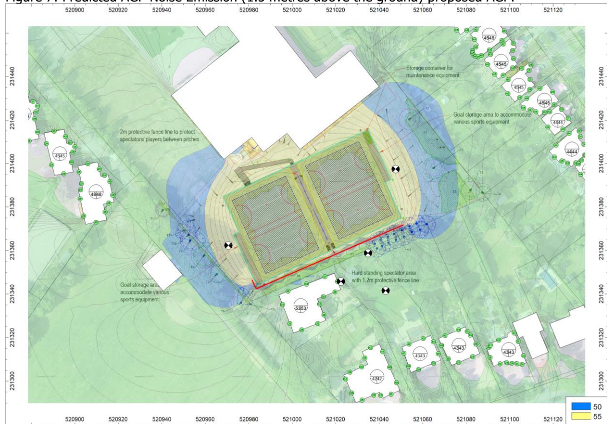
Figure 7: Predicted AGP Noise Emission (1.5 metres above the ground) proposed AGP.
