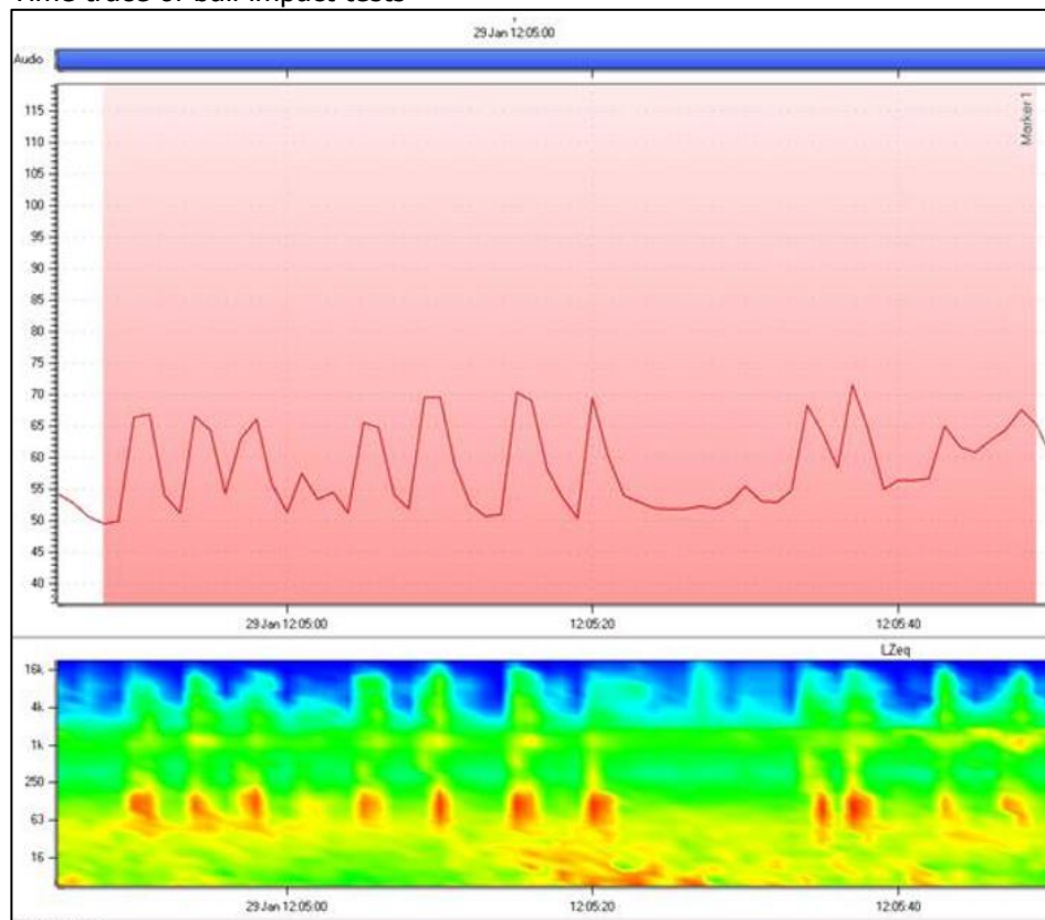
Figure 11: Time trace of ball impact tests
