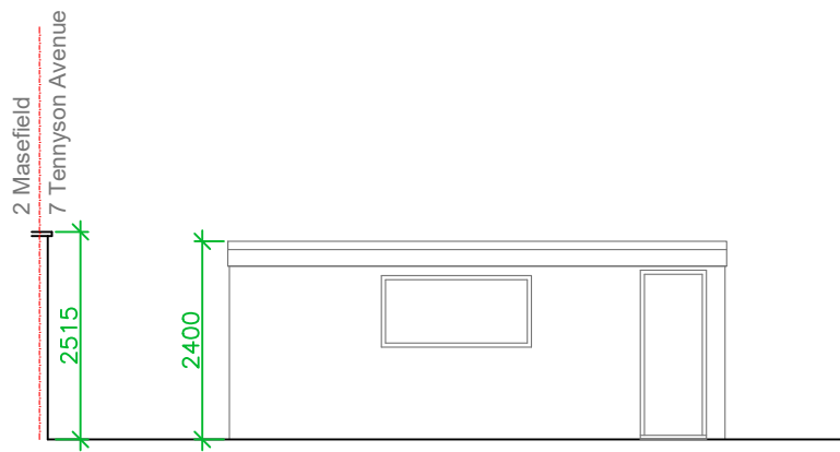
SOUTH ELEVATION AS EXISTING
