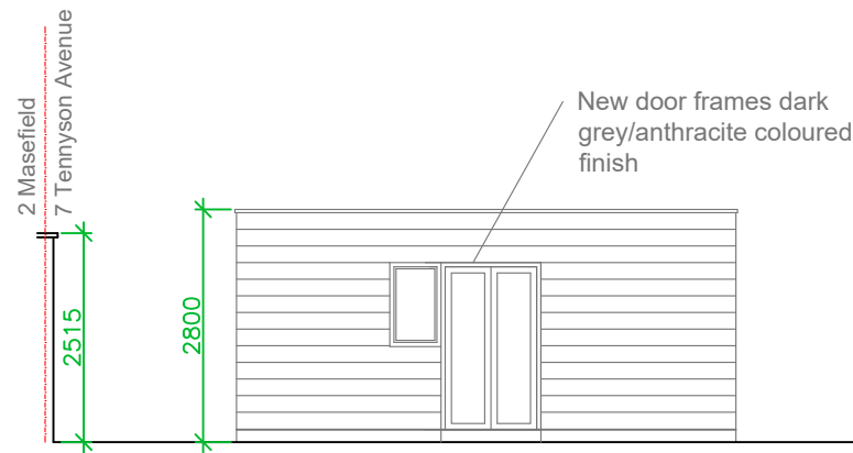
SOUTH ELEVATION AS PROPOSED
