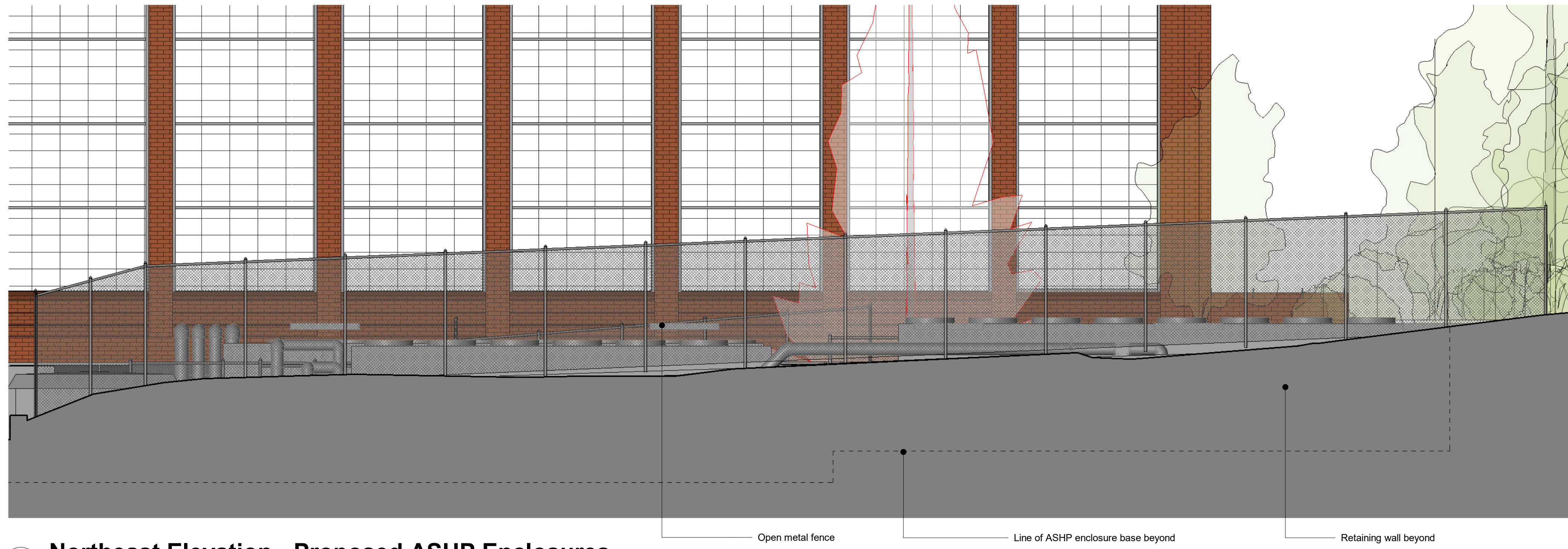
2 Northeast Elevation - Proposed ASHP Enclosures
