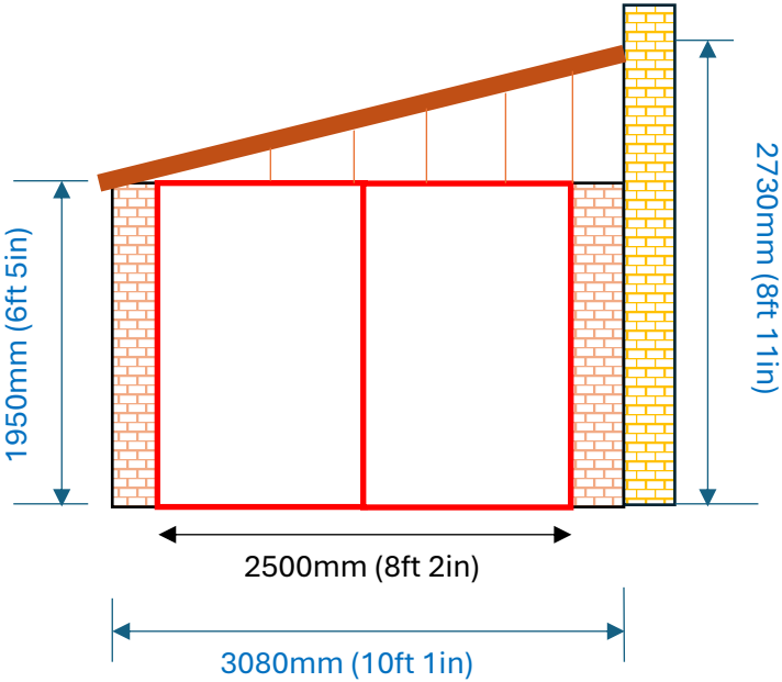
FRONT ELEVATION
