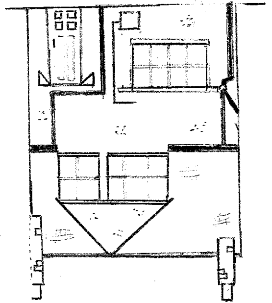
Front 1:100
