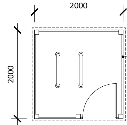
BIKE STORE PLAN
