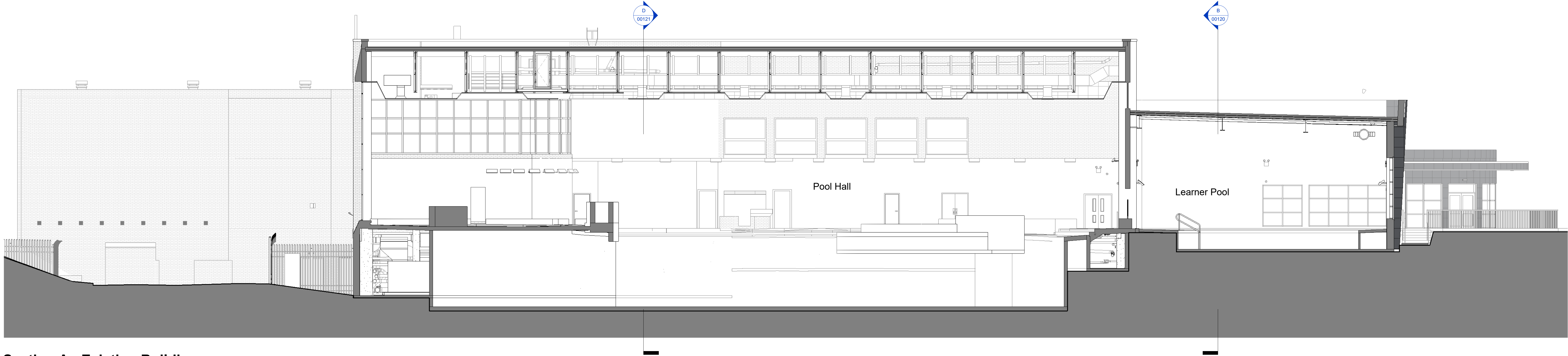
Section A - Existing Building 1 : 100
