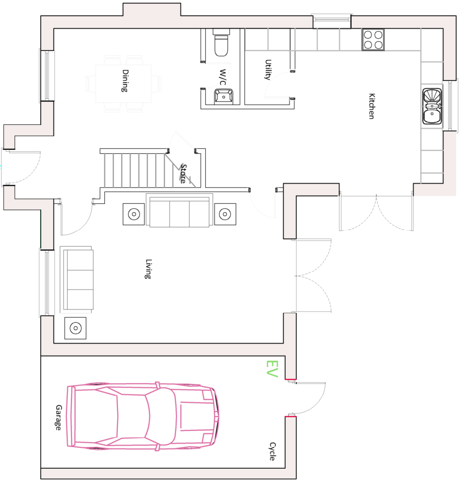
Ground Floor
