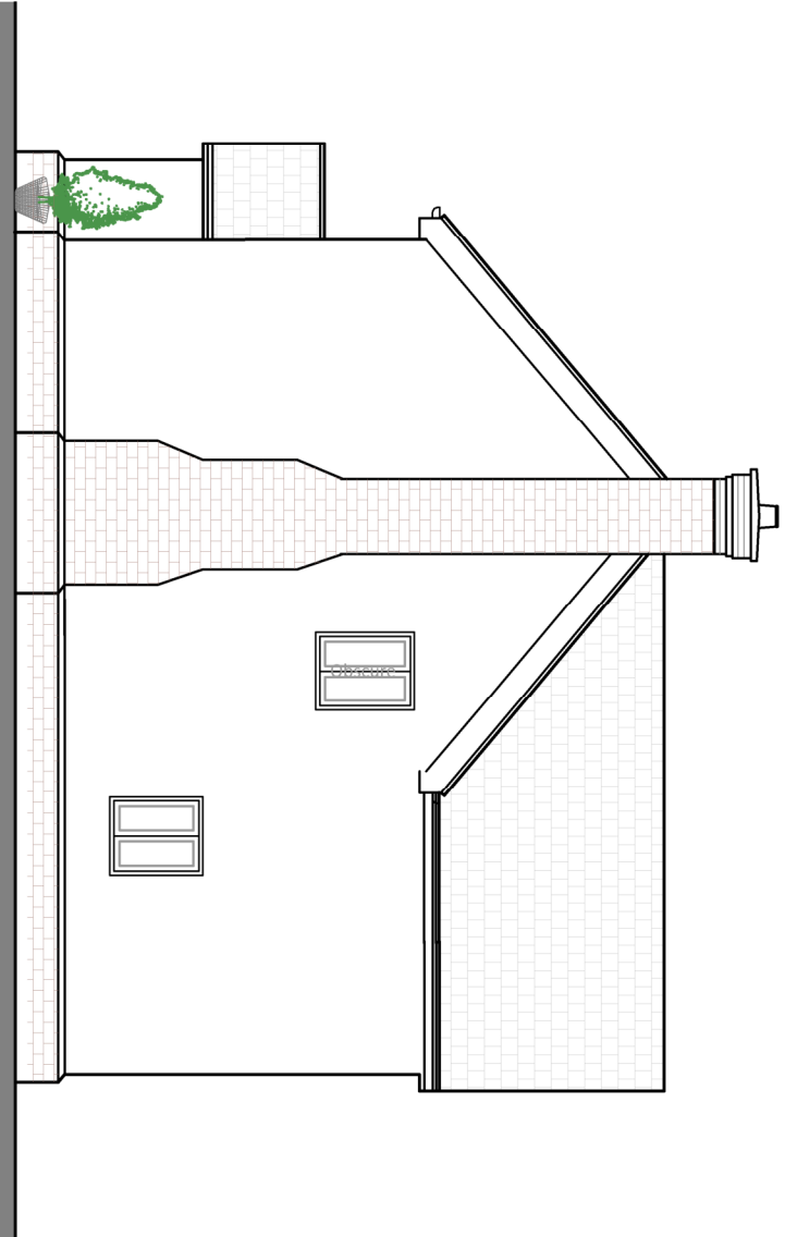
Side (NW) Elevation
