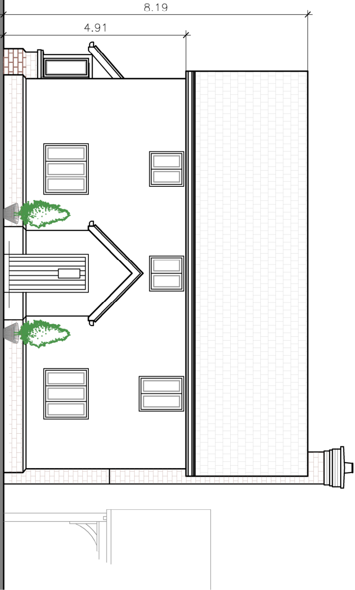
Front (NE) Elevation
