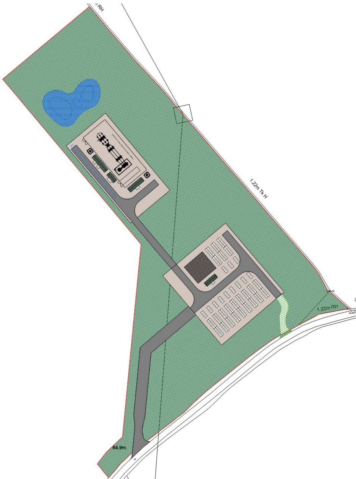
Figure 3: Proposed Site Layout Plan
