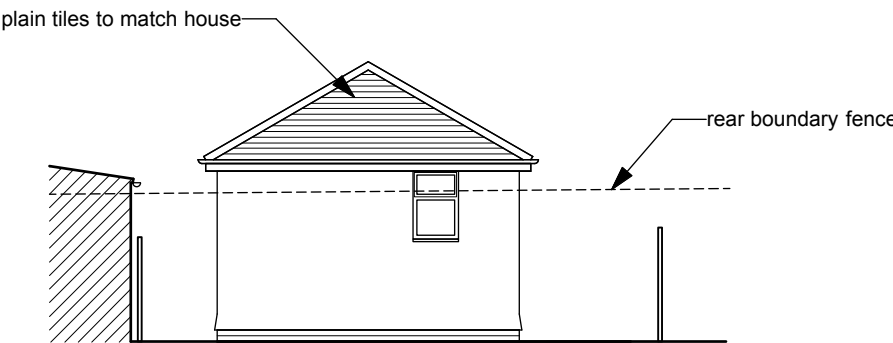
Existing North Elevation (1:100)
