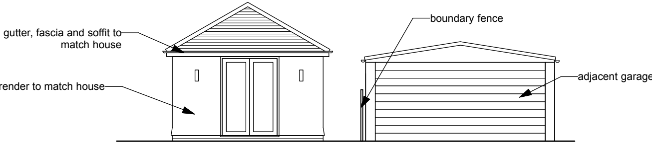
Existing South Elevation (1:100)
