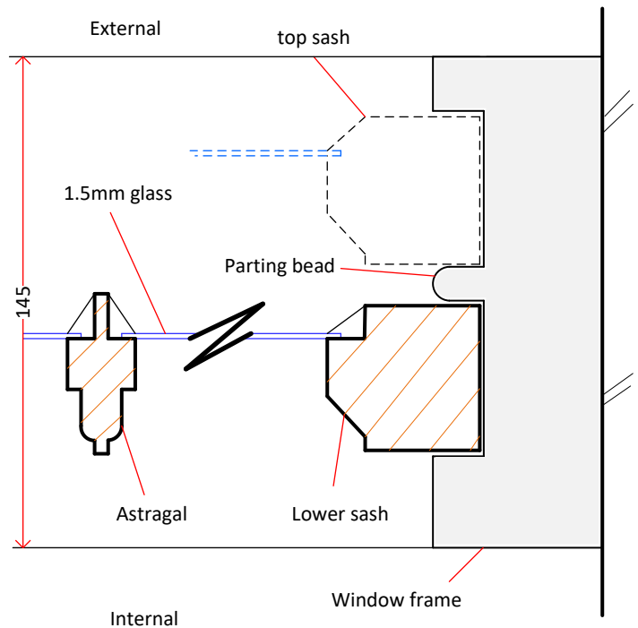
EXISTING
