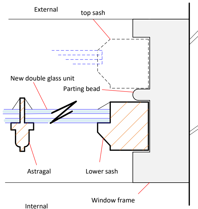
PROPOSED
