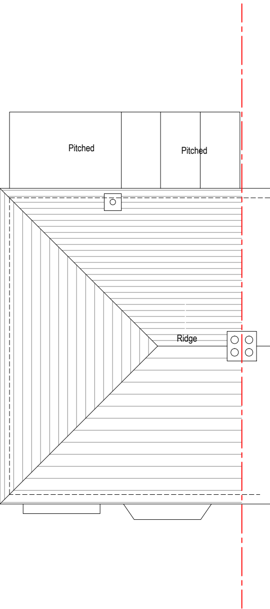
01 006 EXISTING ROOF PLAN 1:100
