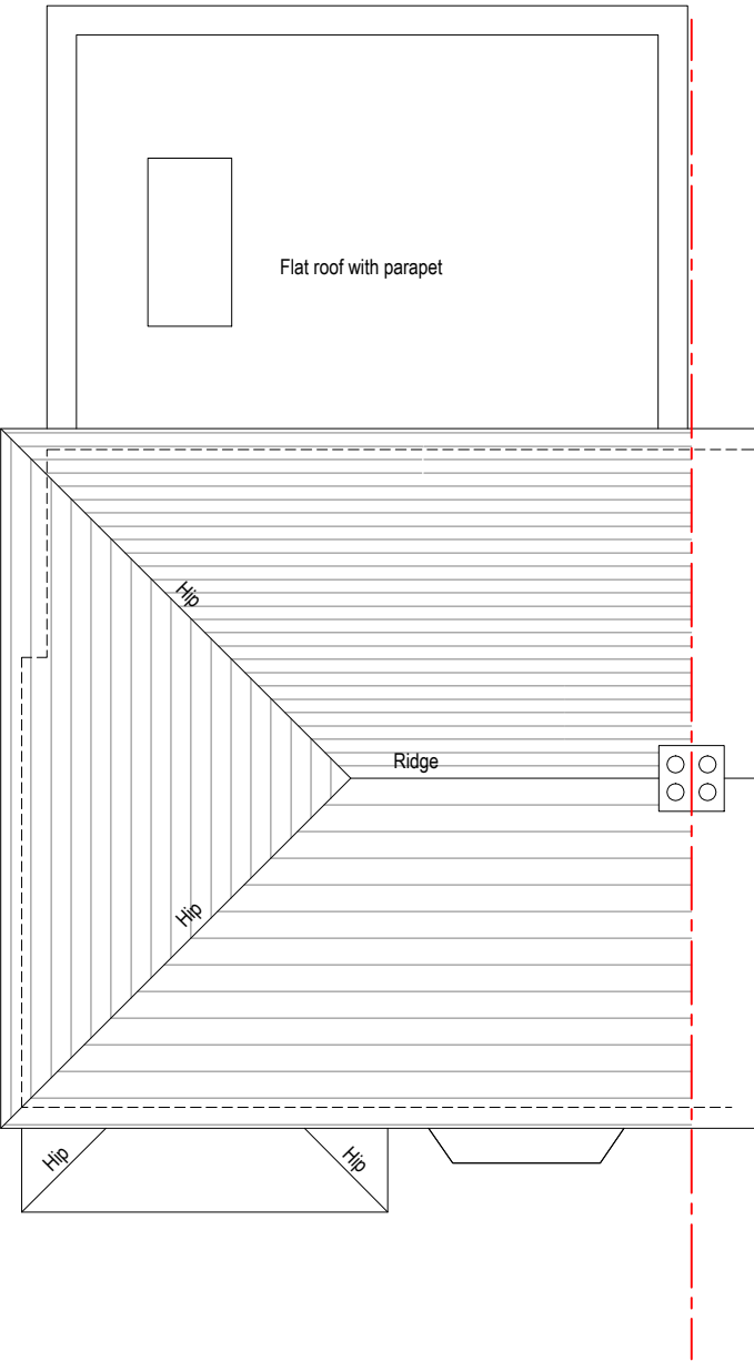
02 004 PROPOSED ROOF PLAN 1:100
