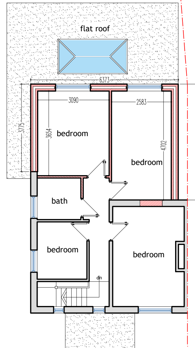
proposed f.f plan
