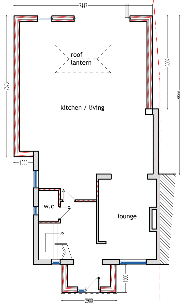
proposed g.f plan
