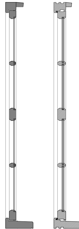
Existing Window Section @ 1:5
