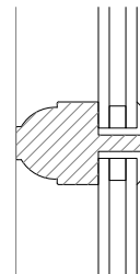
Proposed Window Profile Detail @ 1:1
