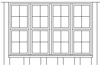
Proposed Window Elevation @ 1:20
