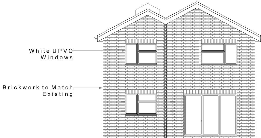
Rear Elevation
