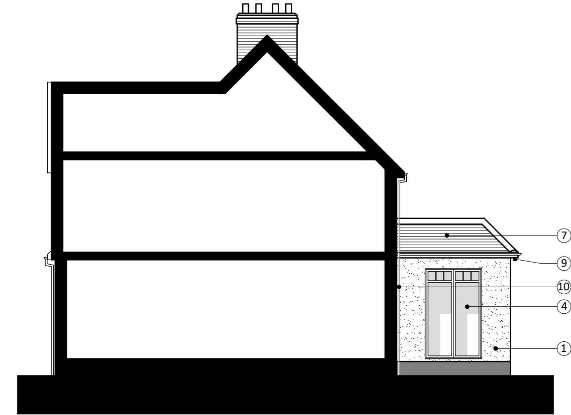
SIDE ELEVATION (D-D)
