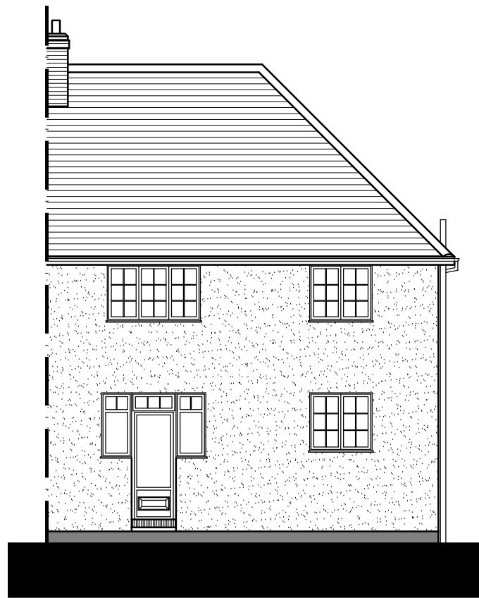
REAR ELEVATION (B-B)
