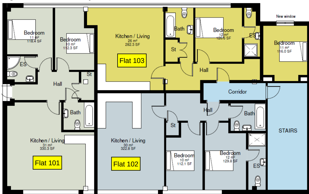
Figure 3: First floor layout
