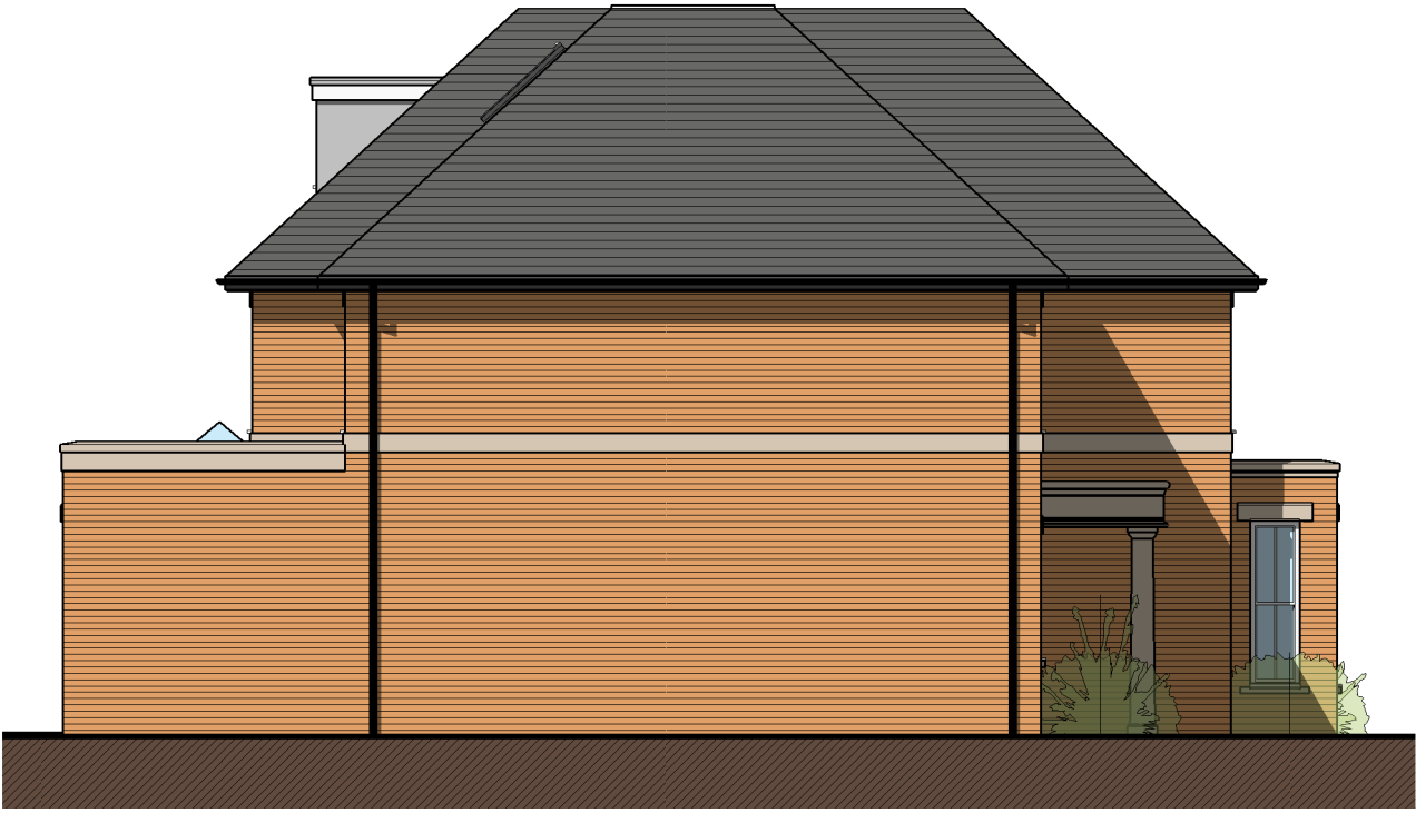
Proposed North West Elevation 1 : 100
