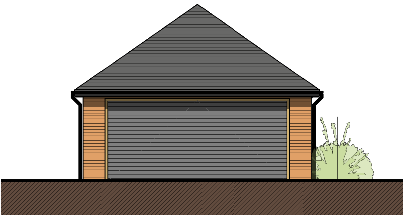
Proposed Front Elevation 1 : 100
