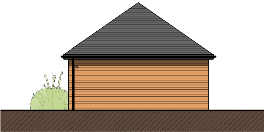
Proposed Side (left) Elevation 1 : 100
