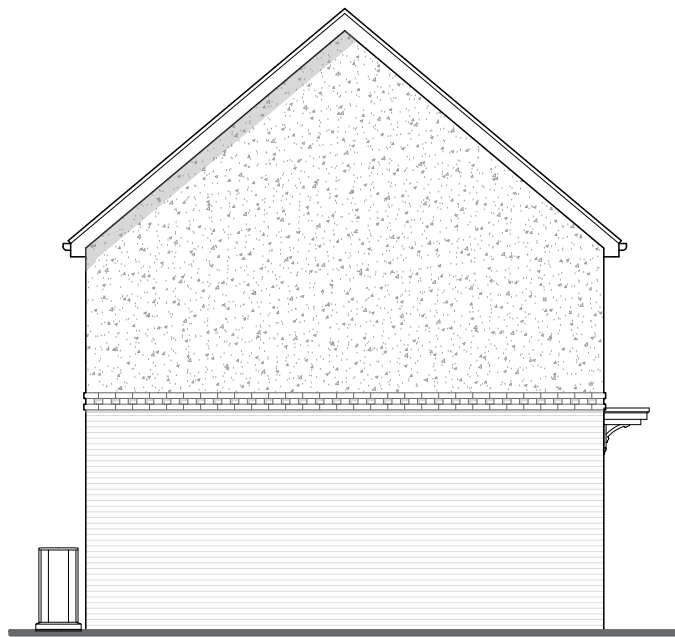
Elevation B Plots 114 As
