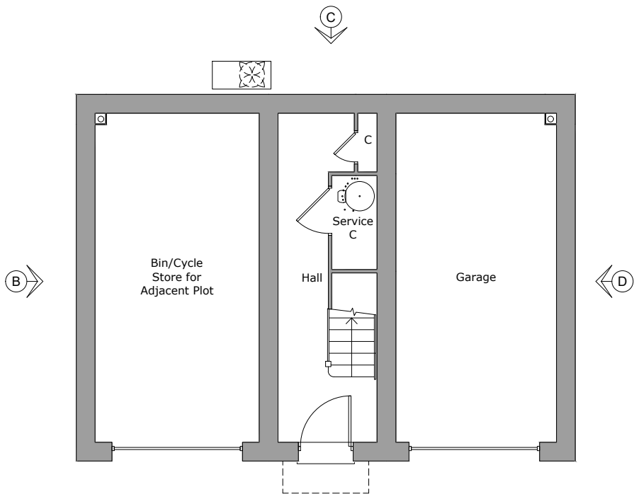
Ground Floor Plan Area 11.4m 2
