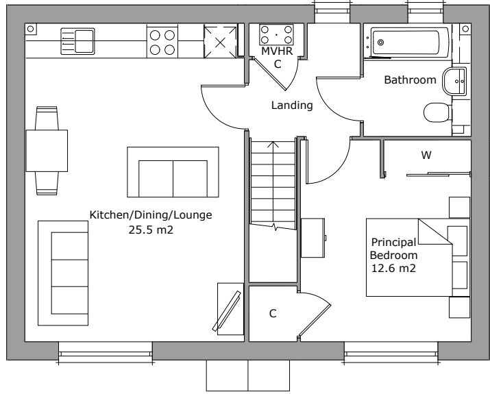
First Floor Plan Area 53.0m 2
