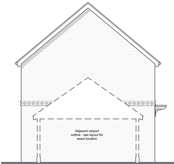
Elevation B Plots 88 As
