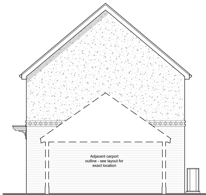
Elevation D Plots 114 As
