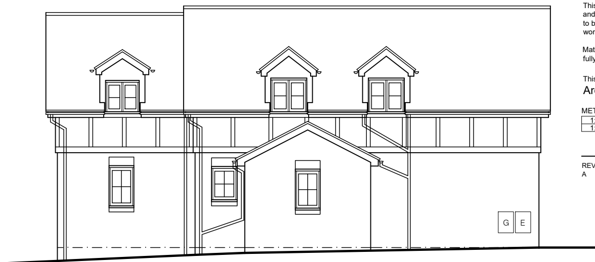
North Elevation
